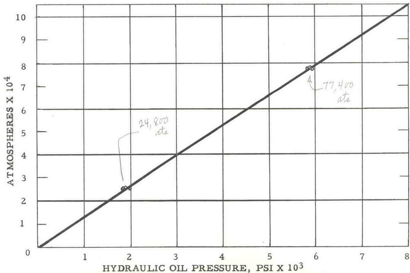
Fig. 2. - Calibration curve for large and small tetrahedral presses
