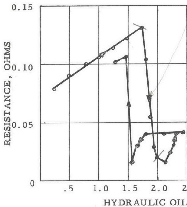
Bismuth transition
