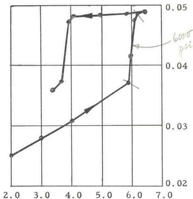
Barium transition
